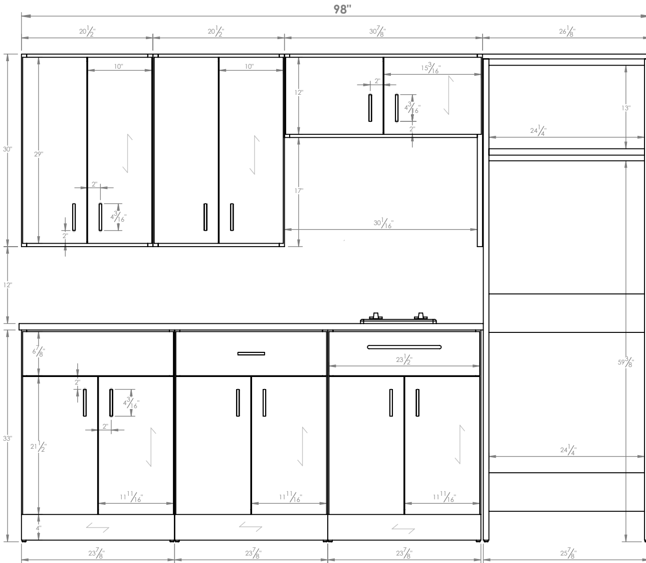
FRONT ELEVATION
