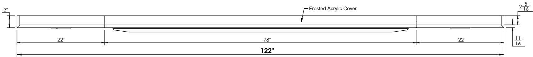
TOP VIEW
