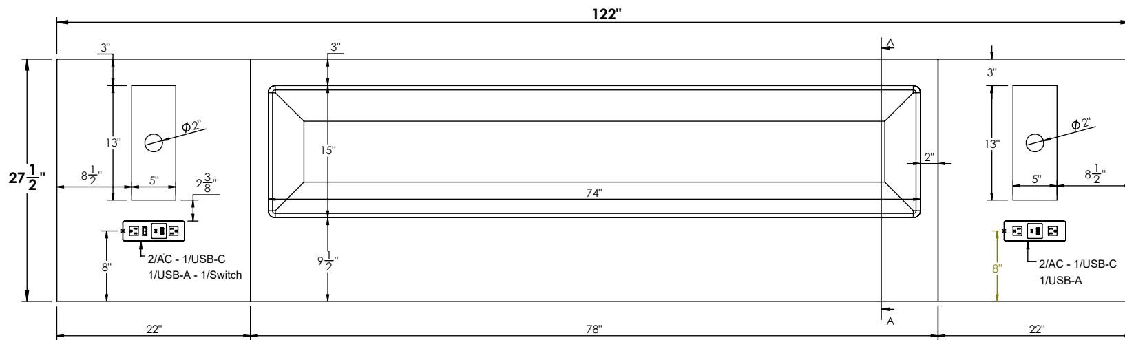
FRONT VIEW
