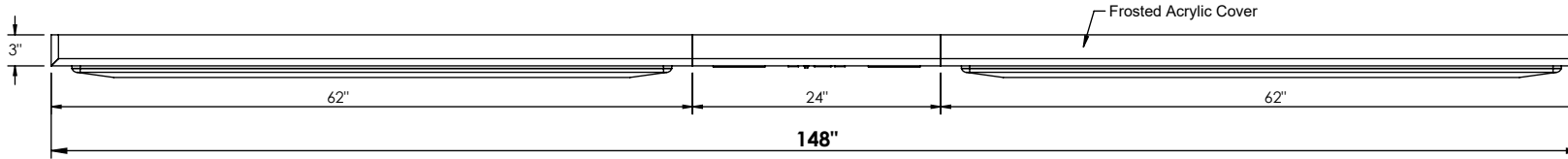
TOP VIEW
